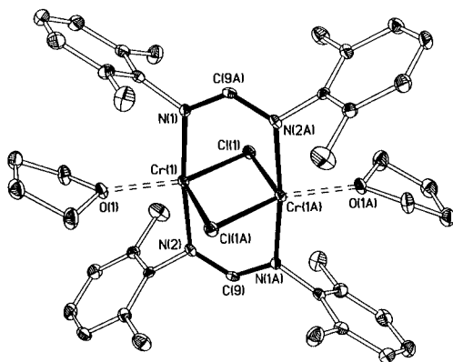
Fig. 3 The molecular structure of \text{Cr}_2(\mu\text{-Cl})_2(\text{DXylF})_2(\text{THF})_2 , 2 . Displacement ellipsoids are drawn at the 30% probability level. Hydrogen atoms omitted for clarity.
