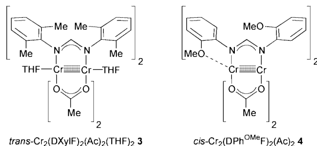
Fig. 1 Schematic drawings of the compounds described in this paper.
